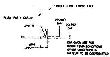
VIEW SCALE: 1/1 INLET CENTERBODY FLOWPATH
